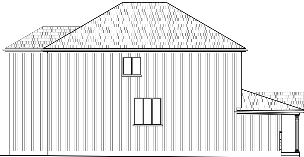
Left Side ( North ) Elevation
